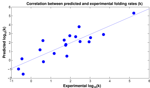
Fig. 3. Scatter plot of log predicted (y-axis) and actual (x-axis) folding rates. The correlation coefficient is 0.87, p \ll 0.001
