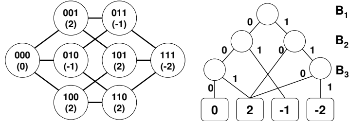
Fig. 1. (Left) A toy example of the protein folding model. This finite-state model corresponds to a 3-residue protein. The state variables and the energy (in parens) are placed inside each node. The state labeled 000 is the unfolded state; the state labeled 111 is the folded state. In our experiments, we considered proteins with between 16 and 107 residues. (Right) A MTBDD of the function mapping the states of the model on the left to their respective energies. Each level of the MTBDD corresponds to one of the three bits/residues ( B_1, B_2, B_3 ), and each path from the root to a leaf maps one (or more) states to an energy. Notice that the MTBDD is smaller than a complete binary tree encoding the same function from states to energies.
