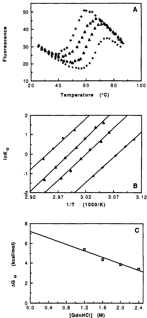
FIGURE 2: Thermal denaturation of CI2 in the presence of low concentrations of GdnHCl, in 50 mM MES, pH 6.3. (A) Intrinsic fluorescence of CI2 as a function of temperature, with (■) 1.2 M GdnHCl, (△) 1.6 M GdnHCl, (▲) 2.0 M GdnHCl, and (+) 2.4 M GdnHCl. (B) van't Hoff plots of the thermal transition curves around the midpoint of the transition, with (■) 1.2 M GdnHCl, (△) 1.6 M GdnHCl, (▲) 2.0 M GdnHCl, and (+) 2.4 M GdnHCl. The solid line indicates the best fit of the data to eq 4. (C) Plot of the free energy of denaturation at 25 °C, calculated from the van't Hoff plots, and using eqs 7-9, versus [GdnHCl]. Linear extrapolation to 0 M GdnHCl results in the free energy of denaturation in the absence of denaturant.
