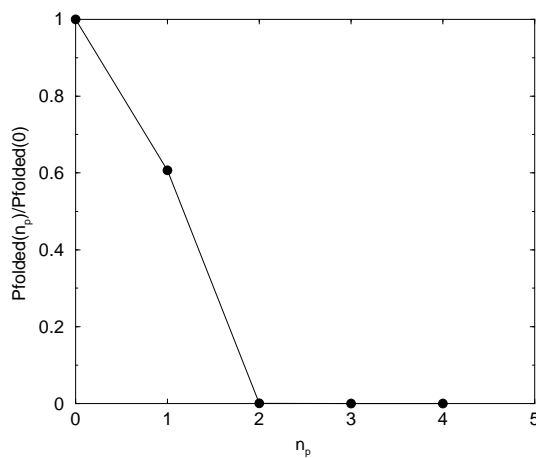
Figure 13: The relative occupancy \frac{P_{folded}(n_p)}{P_{folded}(0)} of the native state shown in Fig. 12(d) by the sequence S_{36} interacting with n_p p-LES 27'-30'.
