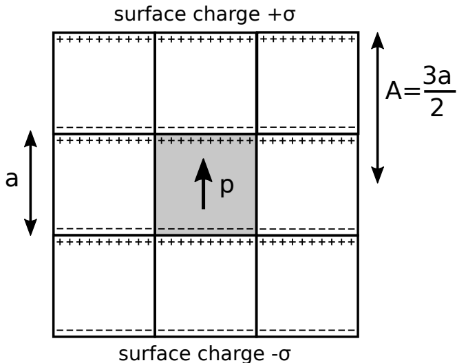
Figure 15: Charge distribution for working out dipole correction. The primary image is shown in gray. Note that the charges cancel at all interior interfaces, leaving surface charges at the top- and bottom boundaries.
