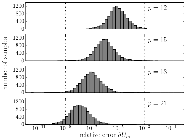
Figure 8: Histogram of the relative error \delta U_m defined in Eq. (19) for different numbers of expansion terms p and a system with N = 10^4 charges.
