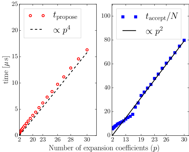
Figure 11: Time per proposal (left) and per acceptance step normalised to N (right) for varying polynomial degrees p and fixed N = 10^5 . The horizontal axes are scaled to highlight the quartic/quadratic dependency on p . All results are obtained on an Ivy Bridge node.
