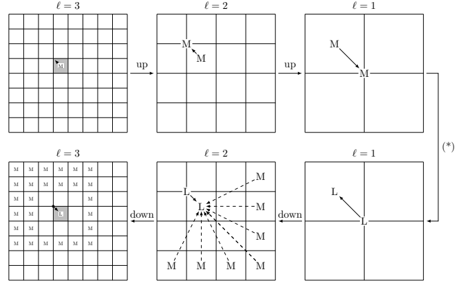
Figure 2: Overview of the FMM field, see Algorithm 3 in Appendix A for details. The translation of multipole expansions \Phi_{\ell,\alpha} in the upward pass is shown in the first row. The second row shows the conversion of multipole expansions in the interaction list into local expansions \Psi_{\ell,\alpha} , which are represented on the next finer level. The asterisk on the right hand side of the figure stands for any additional operations on the coarsest level to account for the boundary conditions (see Section 2.2.1).
