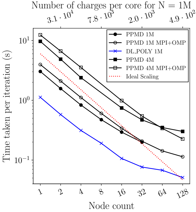
Figure 16: Strong scaling comparison between our FMM implementation (labelled as “PPMD”) and DL_POLY FFT based SPME method. The time per Velocity Verlet step is shown for systems containing N = 10^6 (1M) and N = 4.0 \cdot 10^6 (4M) charges.
