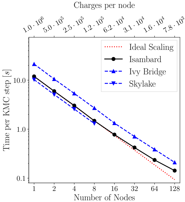
Figure 12: Strong scaling experiment: time per KMC step plotted against number of compute nodes for N = 10^6 charges.
