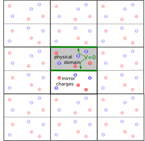
Figure 4: Computational domain used for zero-potential Dirichlet boundary conditions V = 0 at the top and bottom of the device, which is highlighted in green. After duplicating the charges in the physical domain (gray background) with mirror charges, the entire computational domain (black box) is replicated periodically.
