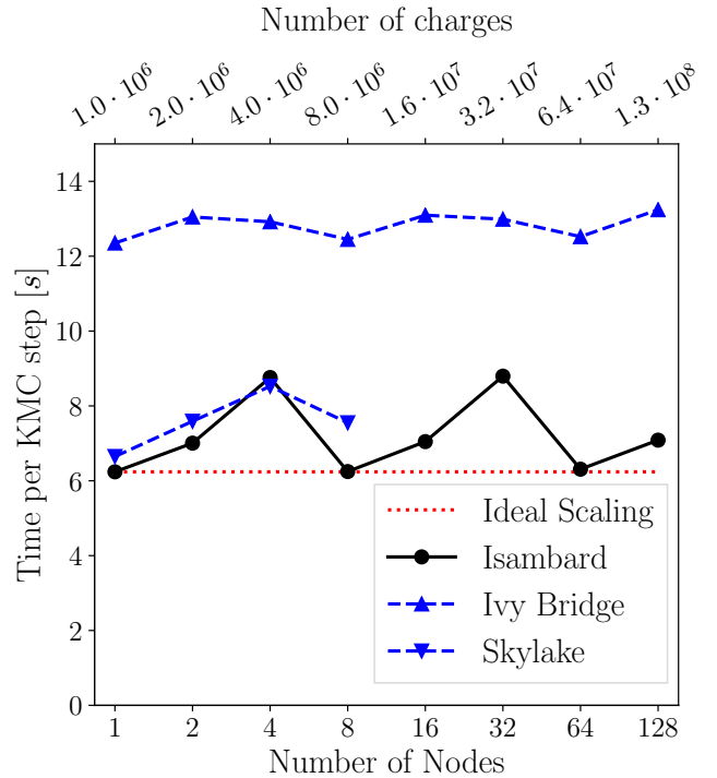
Figure 13: Weak scaling experiment; time per KMC step plotted against number of nodes.
