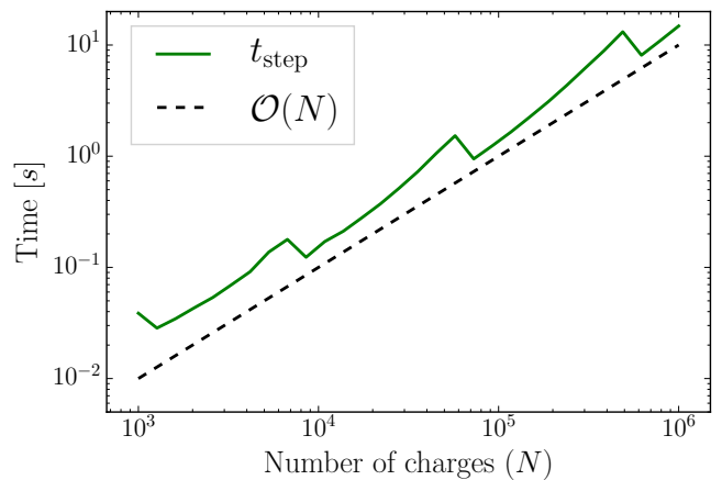
Figure 10: Total time per KMC t_{\text{step}} estimated using Eq. (21) and the numerical values for t_{\text{propose}} and t_{\text{accept}} in Fig. 9, which were obtained on a single Ivy Bridge node. The straight dashed line shows ideal linear scaling with the number of charges N .
