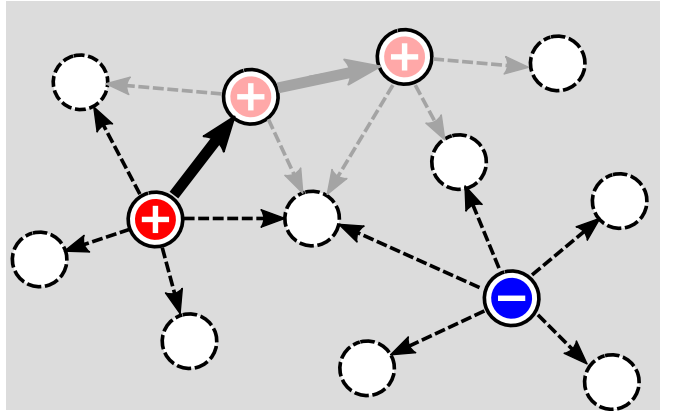
Figure 1: Schematic sketch of one KMC step, which consists of calculation of the propensities for all possible hops (dashed arrows) and moving one particle to a new site after accepting a particular hop (solid arrows). Subsequent steps are shown as gray arrows.
