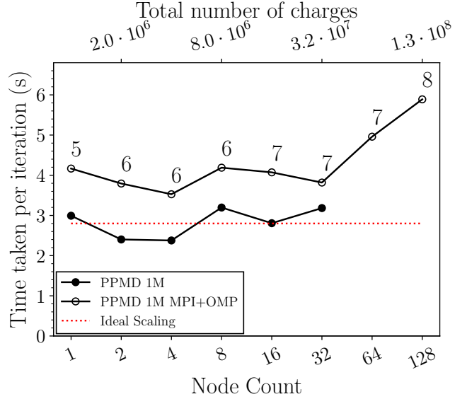
Figure 18: Weak scaling of the time per Velocity Verlet step for the standard FMM implementation. Floating numbers indicate the number of levels in the octal tree.
