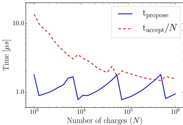
Figure 9: Time per proposed move t_{\text{propose}} and time for accepting a proposal per particle t_{\text{accept}}/N as a function of the number of charges. All results were obtained on a single Ivy Bridge node. The fluctuations in t_{\text{accept}}/N are discussed in the main text.
