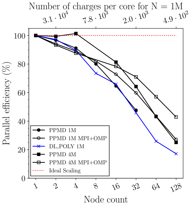
Figure 17: Strong parallel efficiency E_S(P; N) as defined in Eq. (22) of the results shown in Fig. 16.
