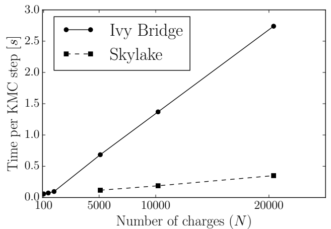
Figure 14: Time per KMC step for \alpha -NPD simulations executed on a single node containing either two Ivy Bridge E5-2650v2 or two Skylake Gold 6126 CPUs. The Ivy Bridge simulations used 4 CPU cores and L = 3 FMM mesh levels. The Skylake simulations used 12 CPU cores and L = 4 mesh levels.
