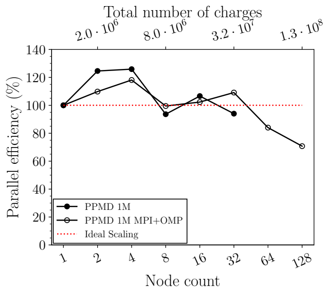
Figure 19: Parallel efficiency as defined in Equation (23) for the weak scaling experiment in Fig. 18.
