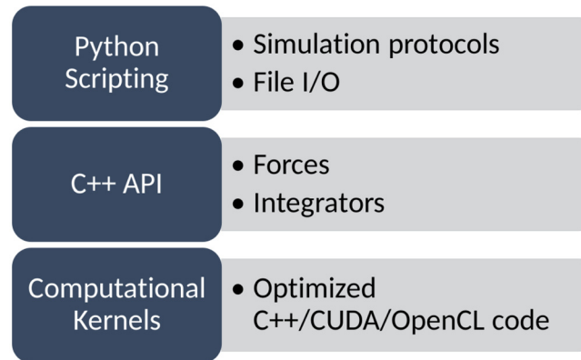
Fig 1. Architecture of OpenMM.
